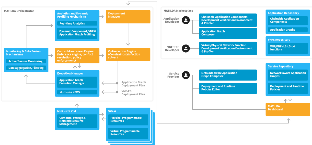
Figure 2. MATILDA 5G High Level Architectural Approach.
